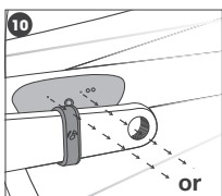
10 Center align cadence band with either marking on sensor as depicted.
