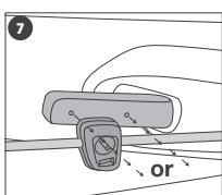
7 Center align speed magnet with either marking on sensor as depicted.
